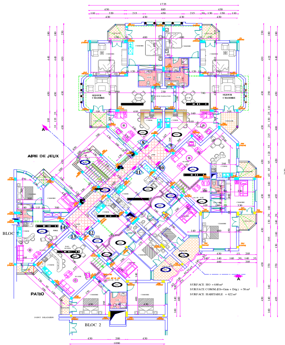
PLAN R +1 ( +400 / +500 )
